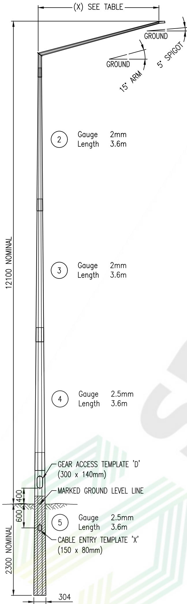
COMPLETE ASSEMBLED VIEW SCALE 1:55
