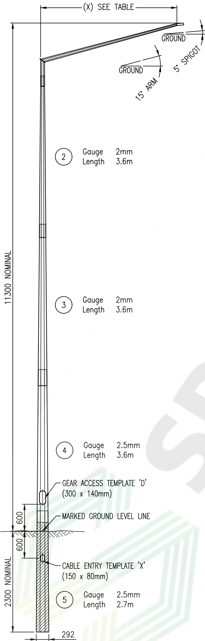
COMPLETE ASSEMBLED VIEW SCALE 1:50
