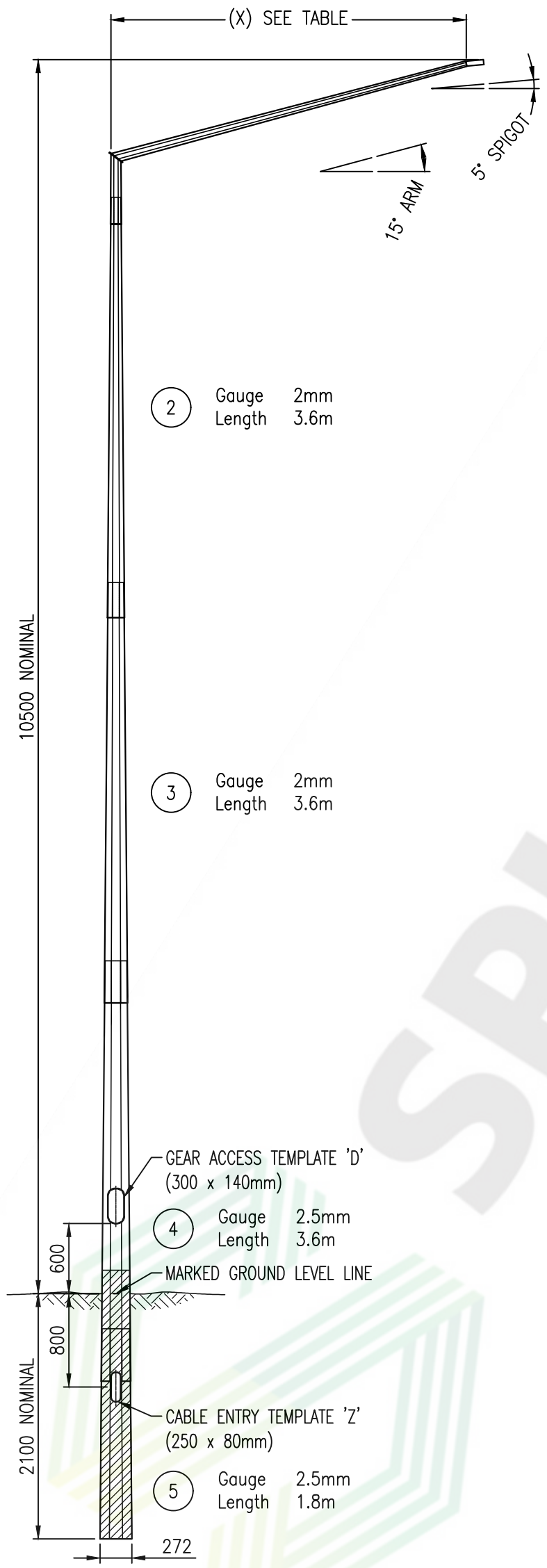
COMPLETE ASSEMBLED VIEW SCALE 1:45
