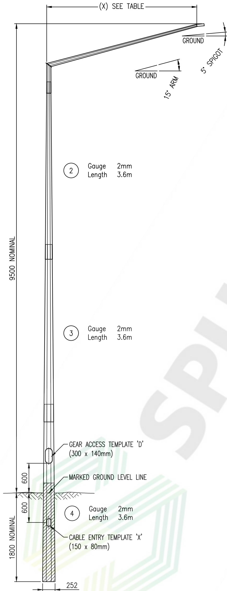
COMPLETE ASSEMBLED VIEW SCALE 1:40
