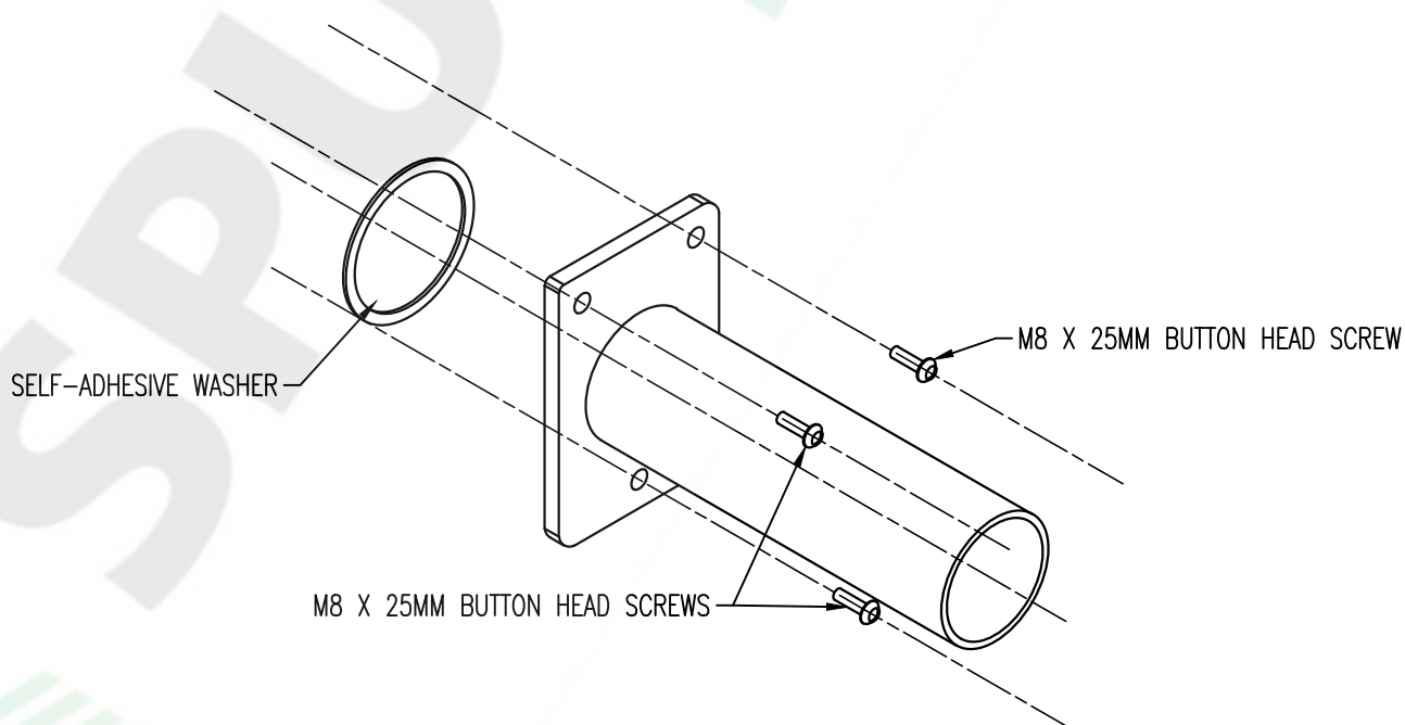
ISOMETRIC VIEW SCALE 1:4
