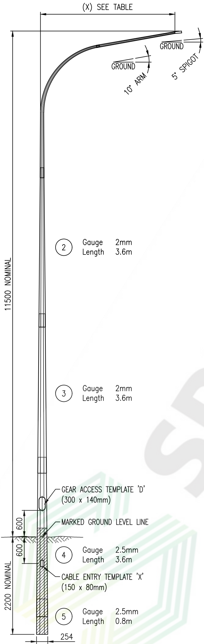
COMPLETE ASSEMBLED VIEW SCALE 1:50
