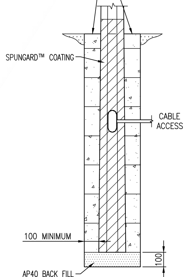
TYPICAL GROUND-PLANTED FOUNDATION SCALE 1:16
