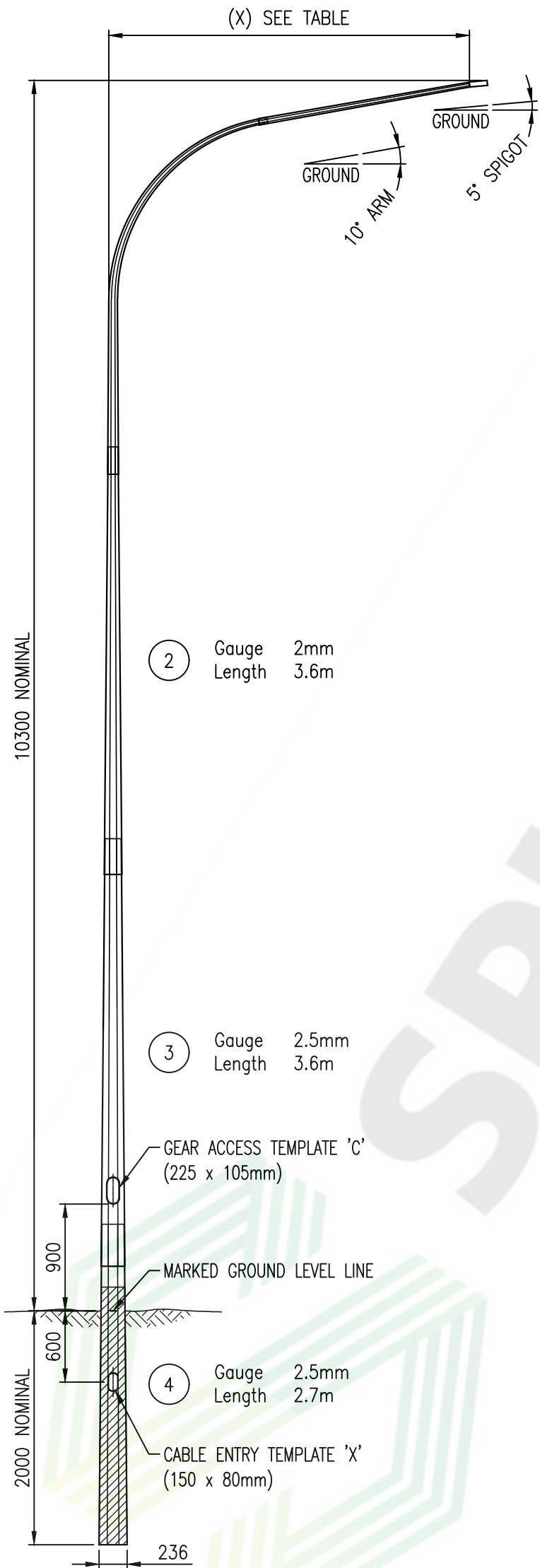
COMPLETE ASSEMBLED VIEW SCALE 1:45
