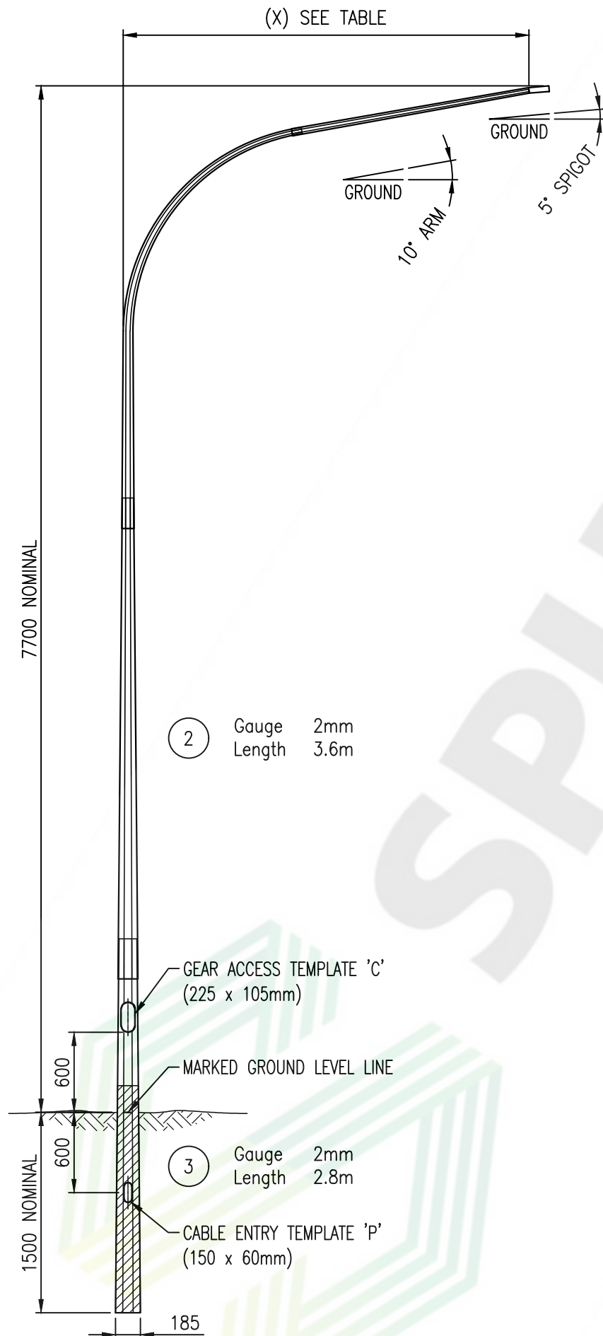
COMPLETE ASSEMBLED VIEW SCALE 1:40
