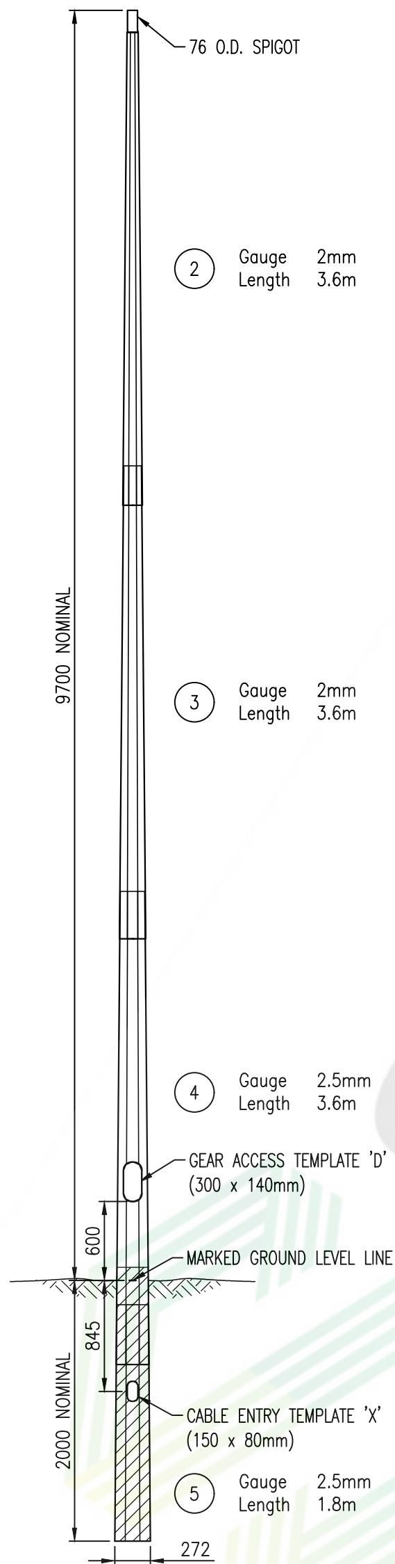
COMPLETE ASSEMBLED VIEW SCALE 1:40
