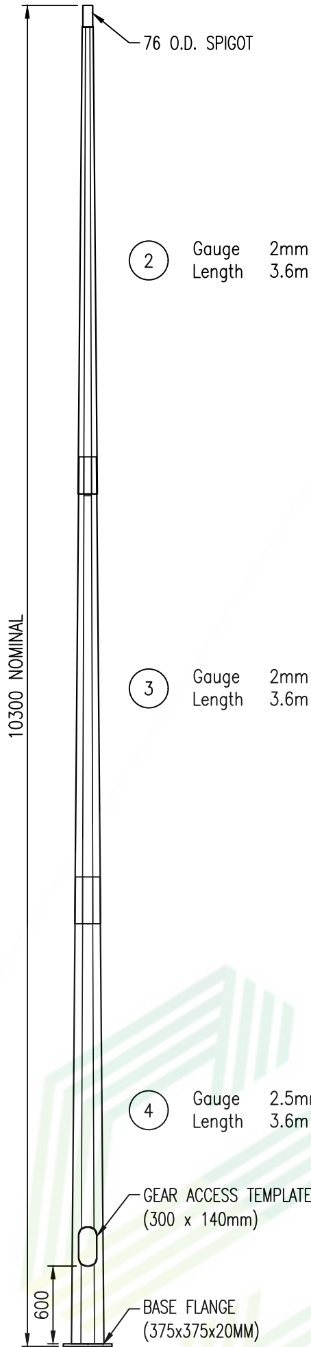
COMPLETE ASSEMBLED VIEW SCALE 1:40
