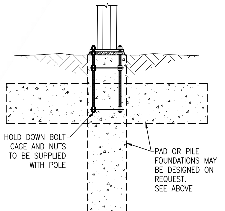
TYPICAL FLANGE-BASED FOUNDATION SCALE 1:20
