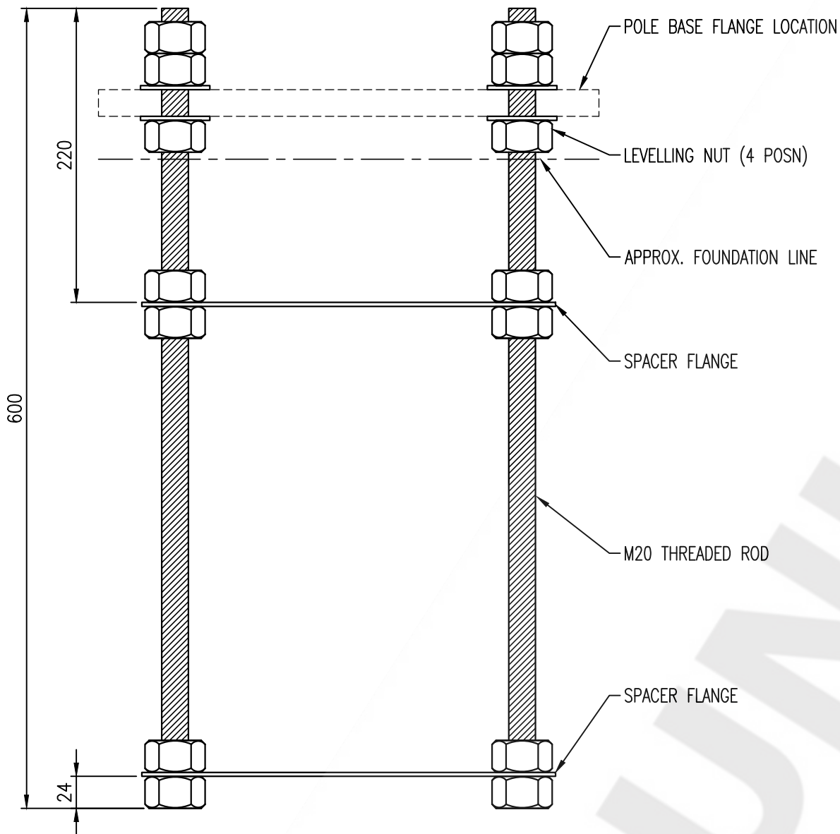
HOLD DOWN BOLT SET ELEVATION SCALE 1:4
