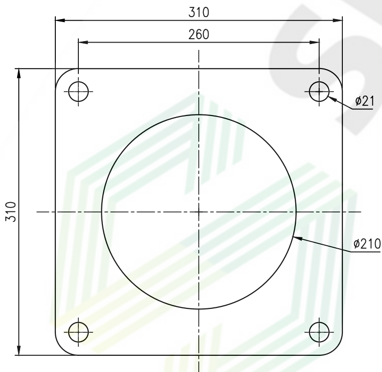
SPACER FLANGE PLAN VIEW SCALE 1:4
