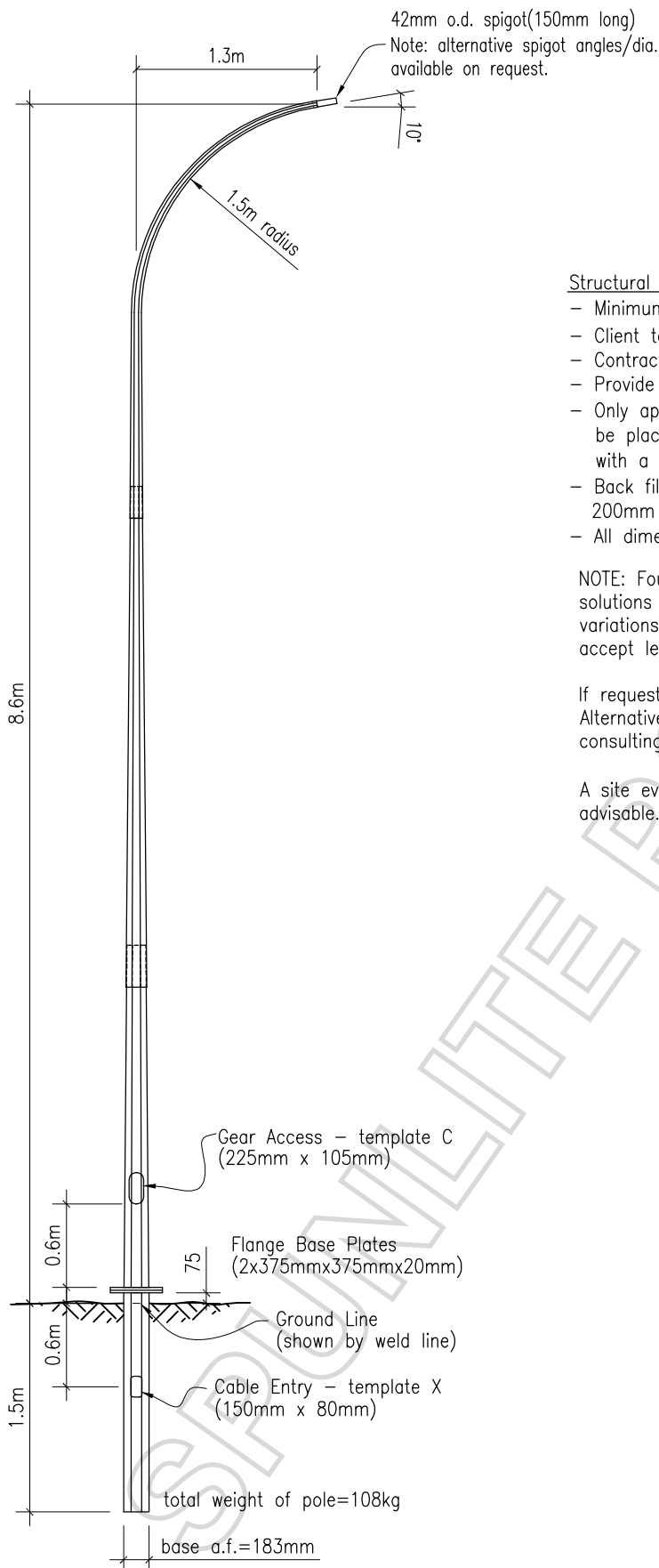
Typical Flange Based Stub Foundation
