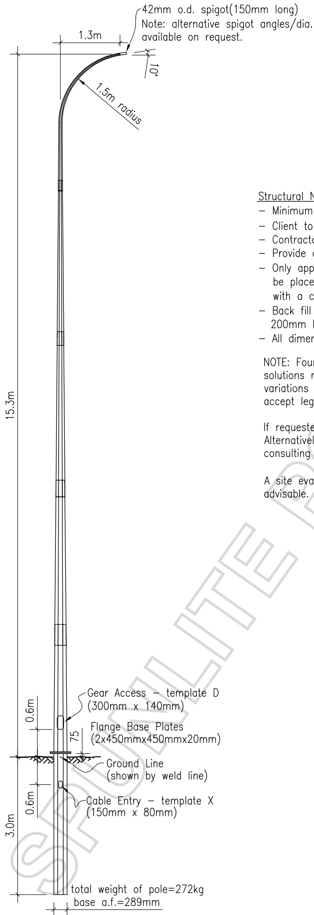
Typical Flange Based Stub Foundation
