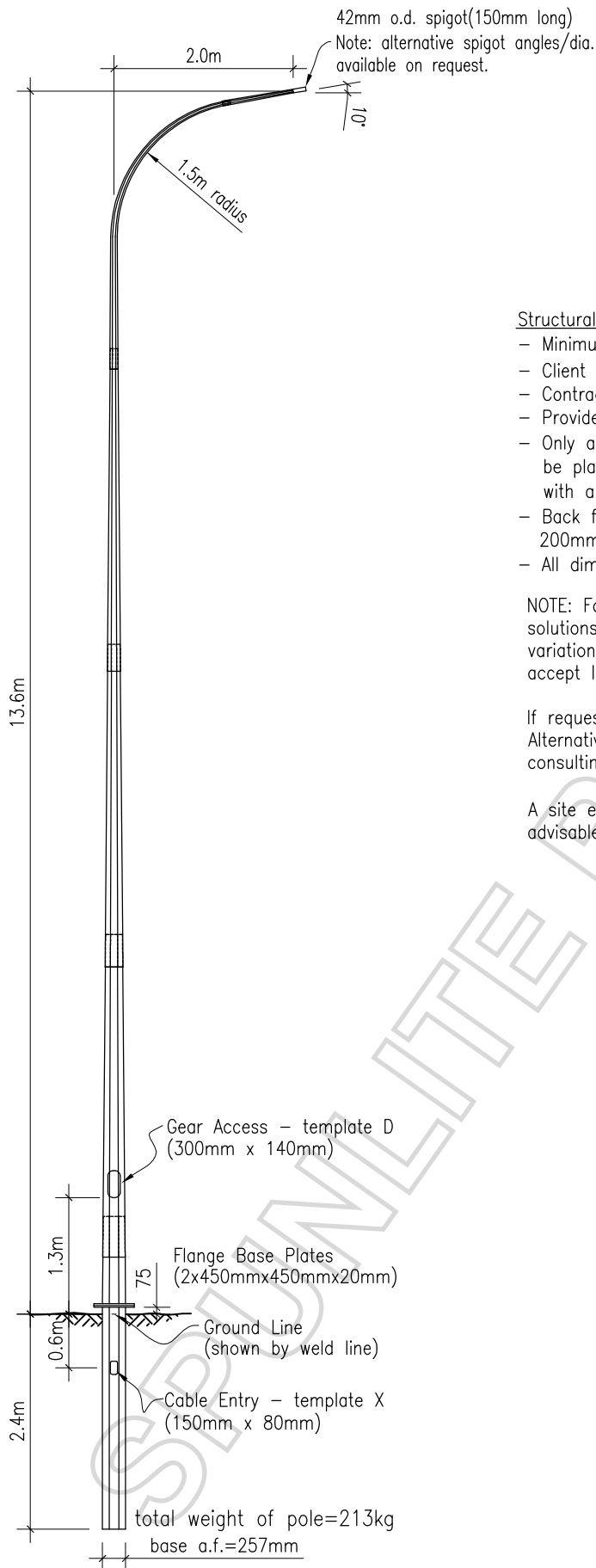
Typical Flange Based Stub Foundation
